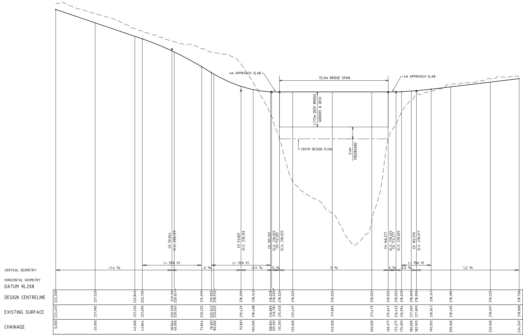
MERRI CREEK ROAD BRIDGE - 50m SOUTH OF ORIGINAL LOCATION
